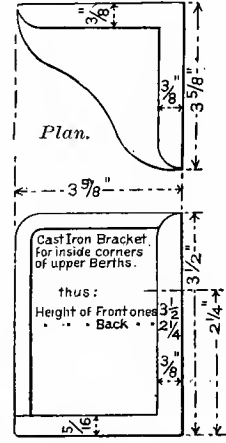
Fig. 4271. Elevation, BERTH CORNER-BRACKET.
